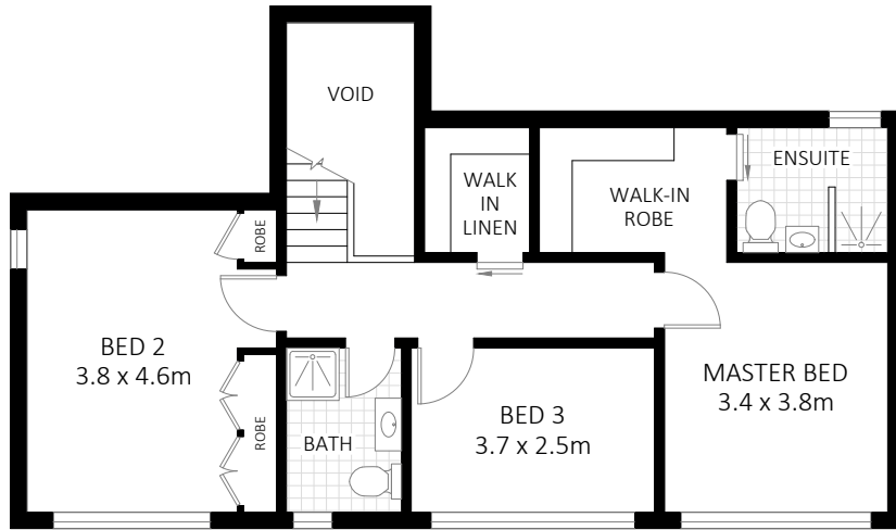
UPPER FLOOR
